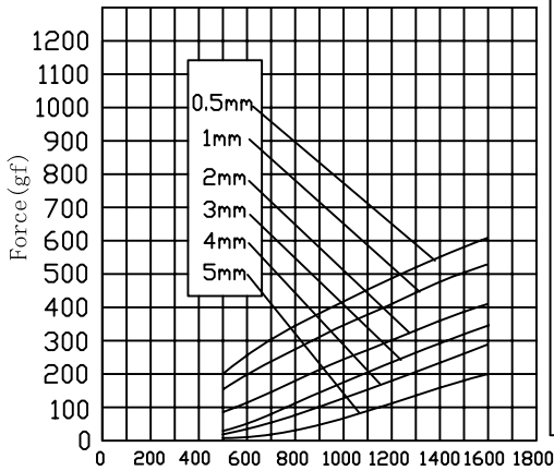
Ampere-turns (AT)
